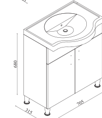
Pera Banyo Dolabi 80 Pera Bathroom Cabinet 80 Pera Badezimmerschrank 80
