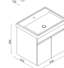
Koza Banyo Dolabi 60 Koza Bathroom Cabinet 60 Koza Badezimmerschrank 60
