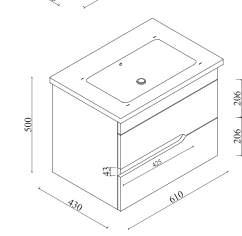
Marmara Banyo Dolabi 65 Marmara Bathroom Cabinet 65 Marmara Badezimmerschrank 65
