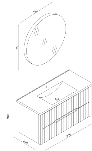
Firuze Banyo Dolabı 100 Firuze Bathroom Cabinet 100 Firuze Badezimmerschrank 100
