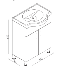
Pera Banyo Dolabi 65 Pera Bathroom Cabinet 65 Pera Badezimmerschrank 65
