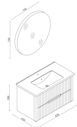
Firuze Banyo Dolabı 85 Firuze Bathroom Cabinet 85 Firuze Badezimmerschrank 85
