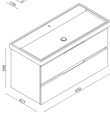
Vega Banyo Dolabı 100 Vega Bathroom Cabinet 100 Vega Badezimmerschrank 100
