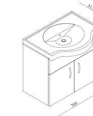
Mercan Banyo Dolabi 80 Mercan Bathroom Cabinet 80 Mercan Badezimmerschrank 80
